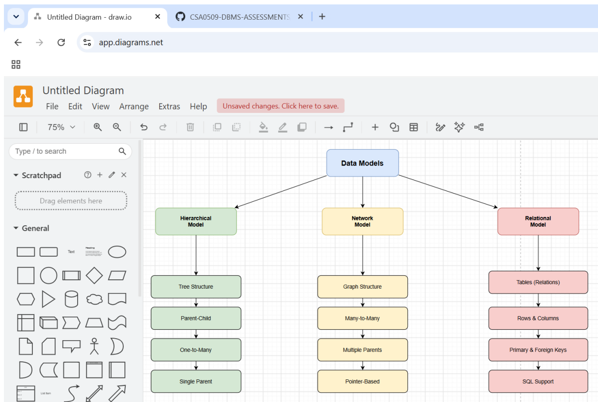
Figure 5: Concept Map Comparing Hierarchical, Network, and Relational Data Models
