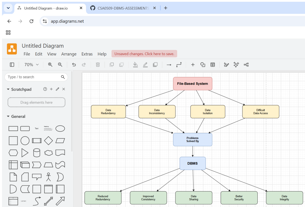
Figure 3: Concept Map Comparing File-Based Systems and Database Management Systems
