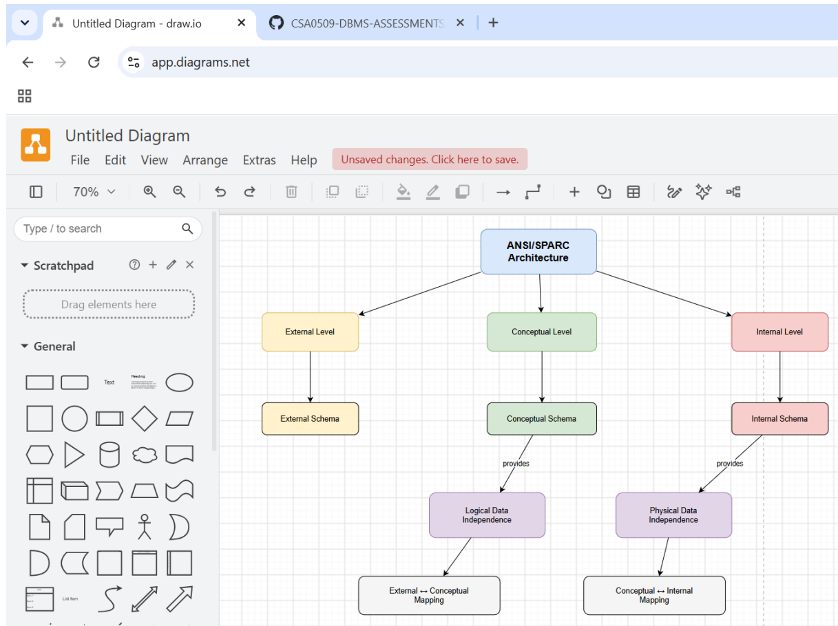
Figure 2: Concept Map of the Three-Level ANSI/SPARC Architecture and Data Independence
